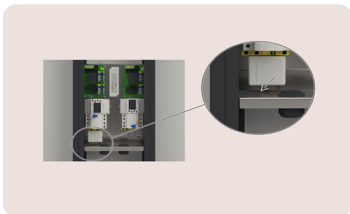
Image 4: View on the cable entry for the network cable
