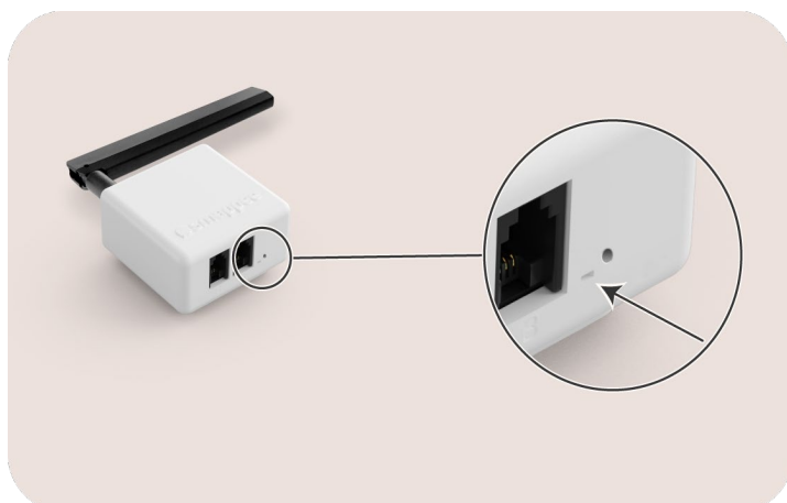
Image 25: Position of the LED on the Smappee 4G Connect (antenna not shown)
