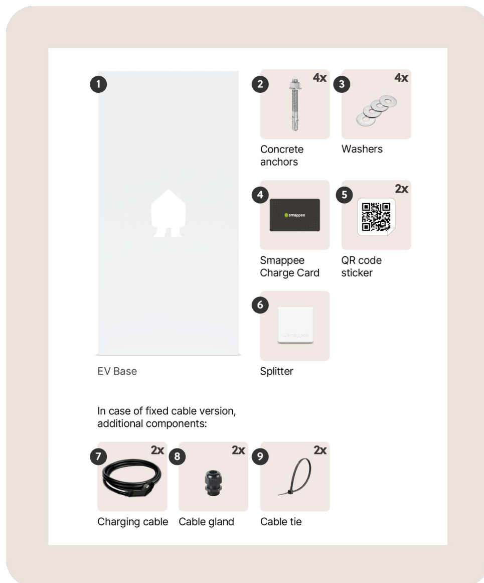
Image 1: What's in the charge box (items 6, 7 and 8 only for EV Base with fixed charging cables)
